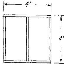
HALF SIZE RETAINING WALL SUBASSEMBLY 1 SHEET OF 1/2"x4'x4' PLYWOOD 3-2"x4" STUDS 2-2"x4" STUDS PLATES 8 REQUIRED
